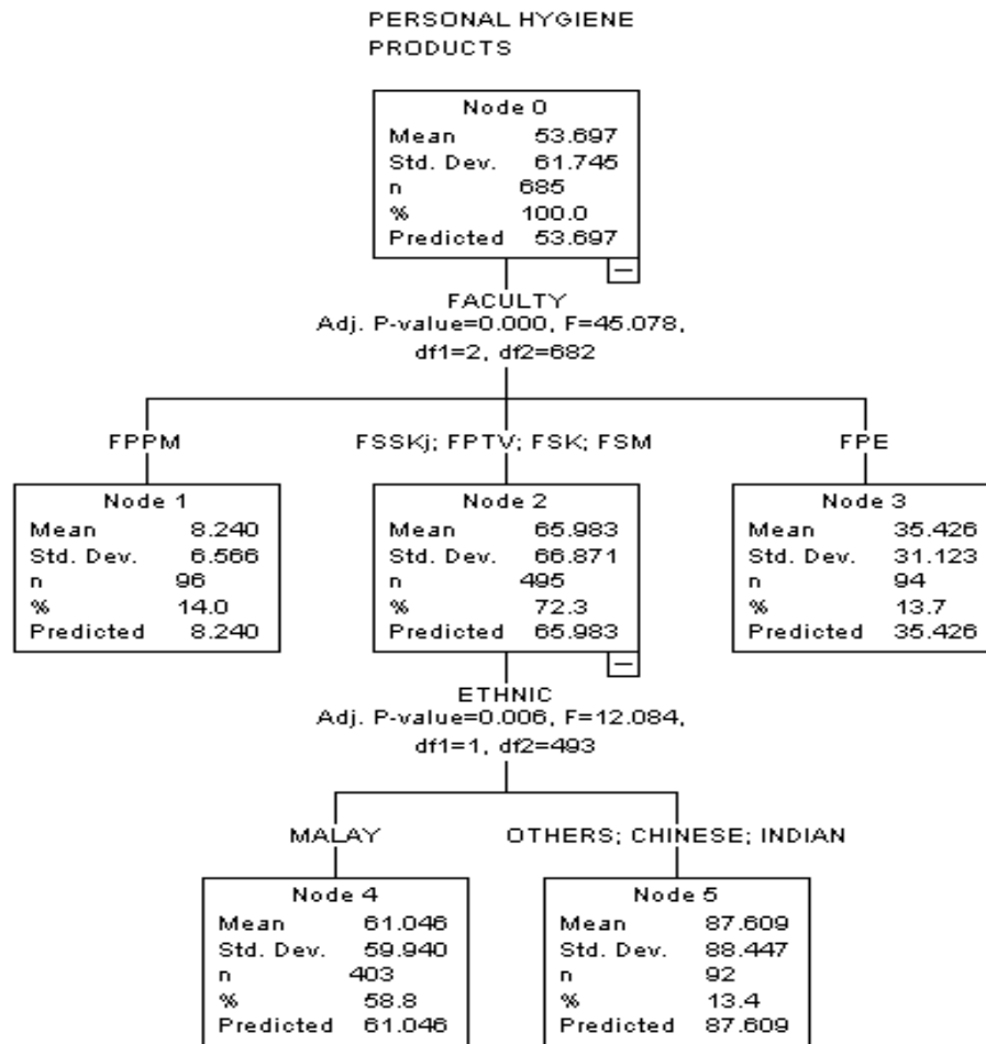
Figure 1: CHAID regression tree
