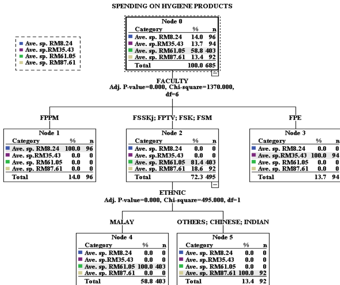
Figure 2: CHAID tree: Personal Hygiene
