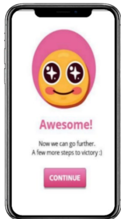
Figure 10: Result interface
